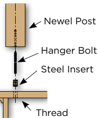
05783 LJ-3004 Newel Mounting Kit
