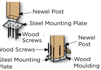
LJ-3006 Newel Mounting Plate for 3" to 3 1/2" newels (Available with plate only.)
