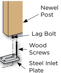
05787 LJ-3005 Keylock™ Newel Post Fastener
