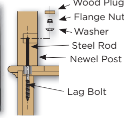
LJ-3070 Threadlock™ Newel Post Fastener
