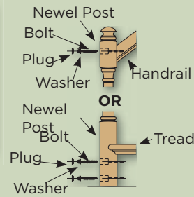
LJ-3078 Rail & Post Fastener
