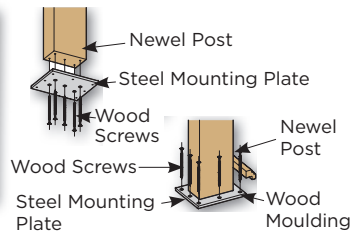
LJ-3006 Newel Mounting Plate for 3" to 3½" newels
