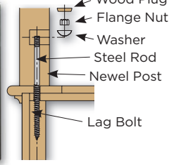
LJ-3008 Sure-Tite™ Newel Fastening System
