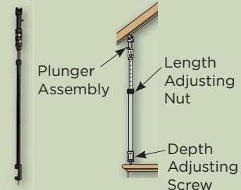
LJ-3047 Telescoping Baluster Marking Tool
