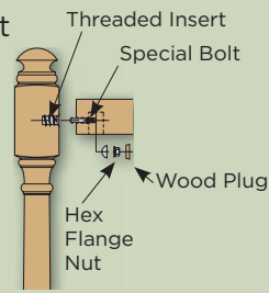
LJ-3078 Rail & Post Fastener
