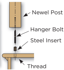
LJ-3004 Newel Mounting Kit
