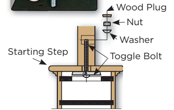
LJ-3071 Toggle Bolt Newel Mounting Kit
