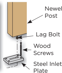
LJ-3005 Keylock™ Newel Post Fastener
